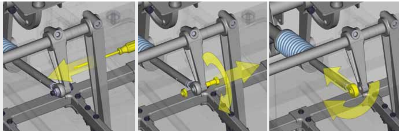
Sample illustrations from the EDGE Video Training Tool showing the adjustment of the shuttle rod on the pinspotter.
